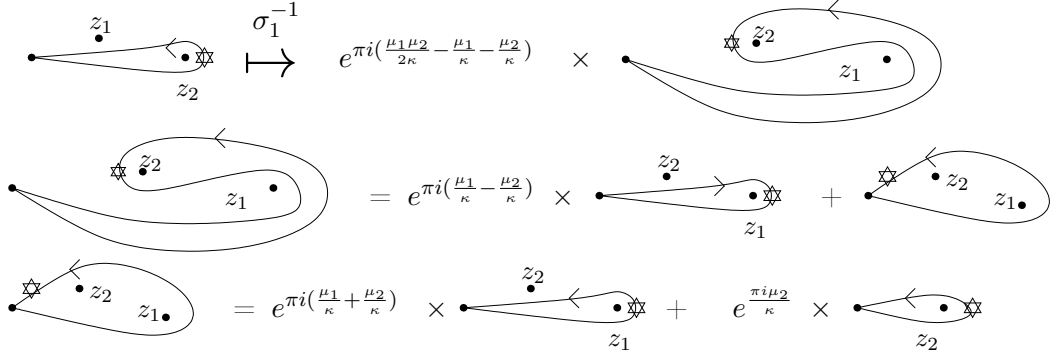
Figure 17: The monodromy of I_k^{(\mathcal{P}_{0,1,0})}
